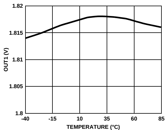
FIGURE 4. OUT1 vs TEMPERATURE
