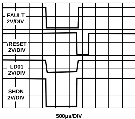
FIGURE 3. SHUTDOWN
