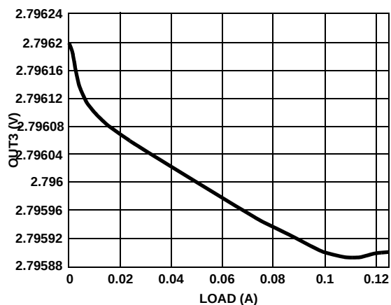
FIGURE 14. OUT3 LOAD REGULATION
