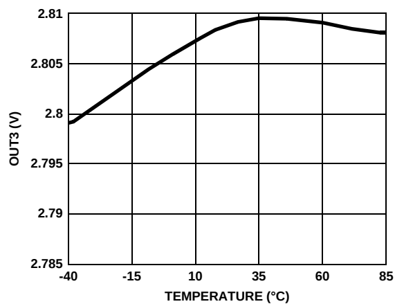
FIGURE 6. OUT3 vs TEMPERATURE
