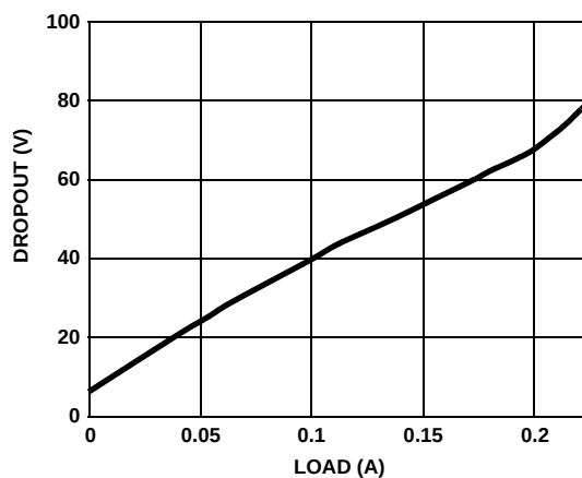
FIGURE 10. OUT2 DROPOUT vs LOAD
