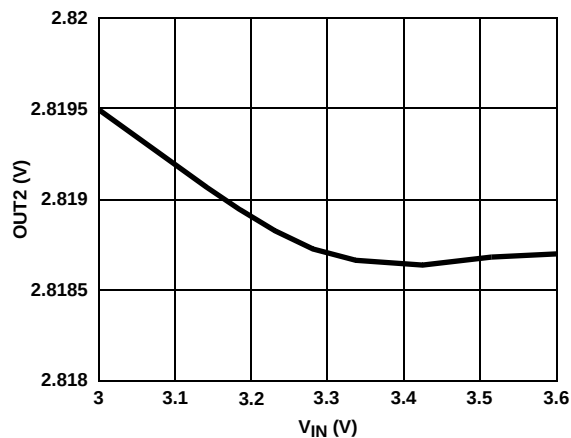
FIGURE 8. OUT2 LINE REGULATION
