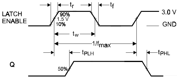
Figure 2. Switching Waveforms
