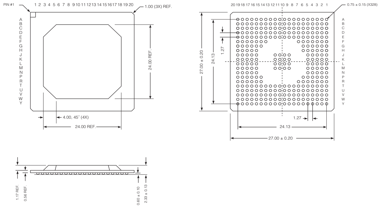
Figure 4-1: Package Dimensions
