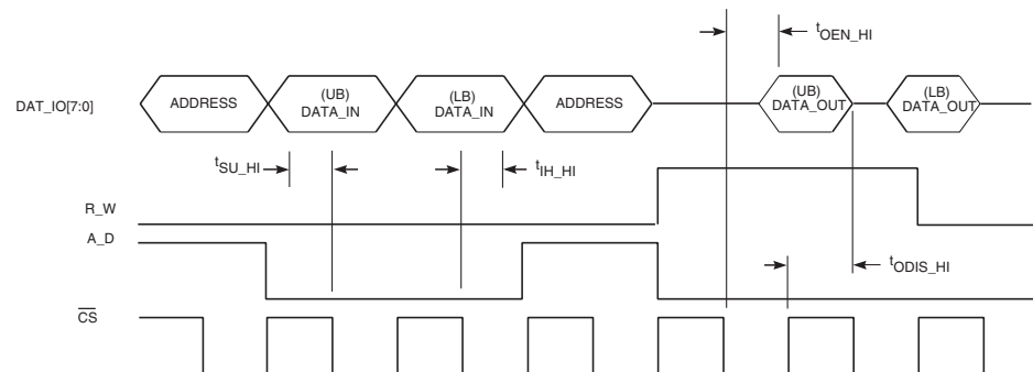
Figure 3-10: Write Cycle to the Parallel Interface
