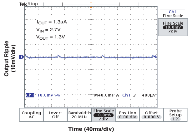
Output Ripple
