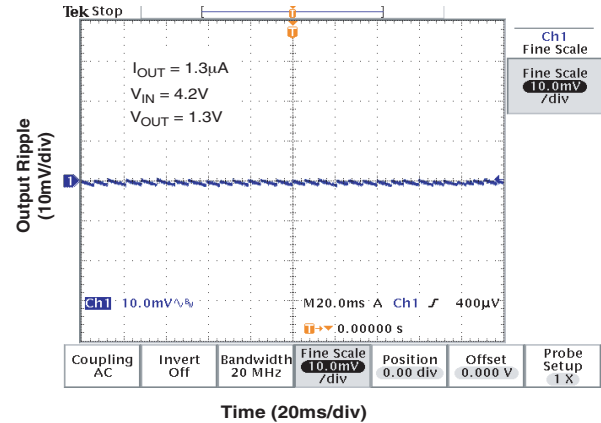
Output Ripple
