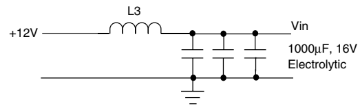
Figure 4. Input Filter
