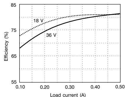
Efficiency (typ)
