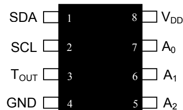
SO (150mil) (DS1631Z)
