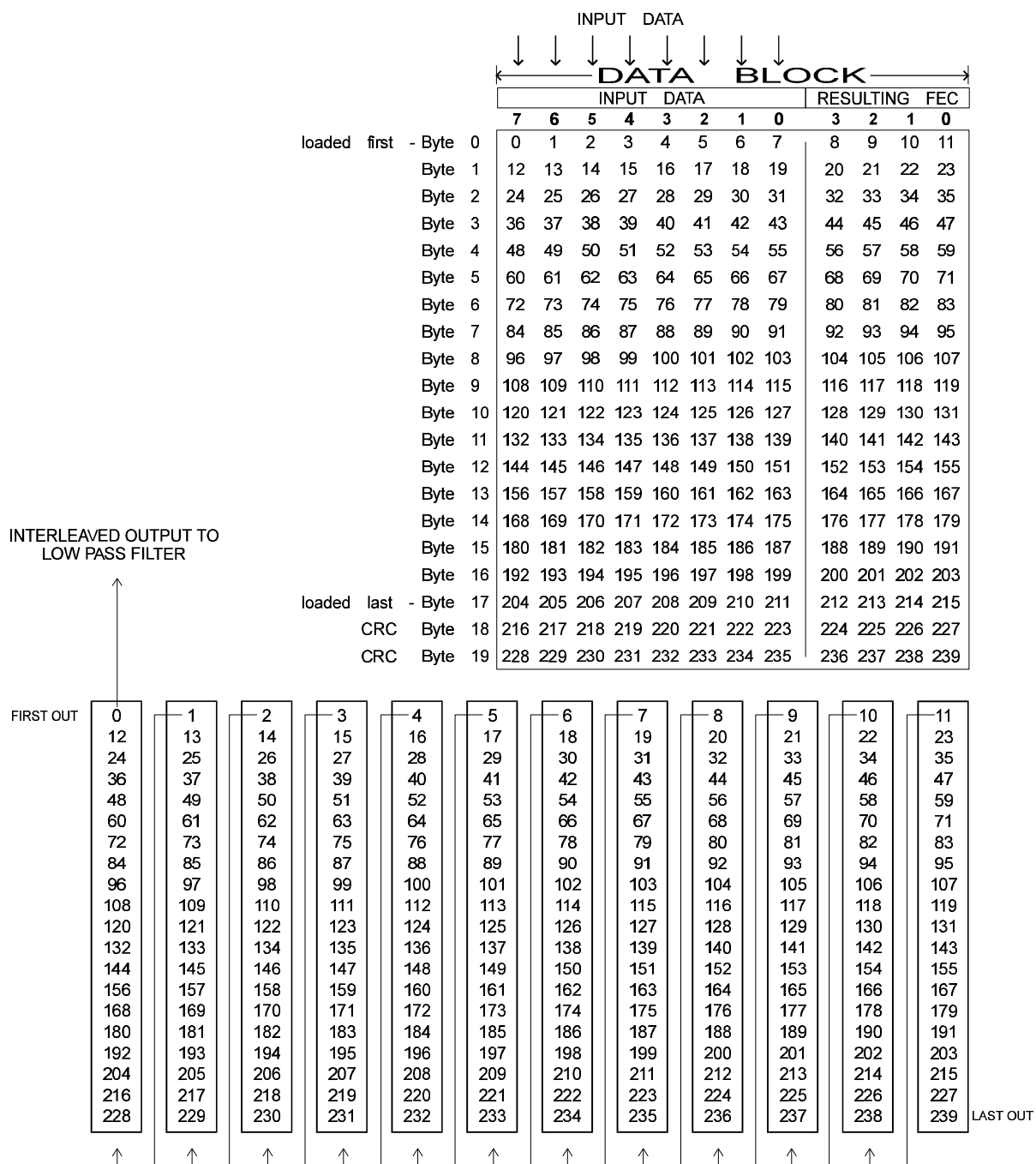
Figure 13 Interleaving - Input/Output
