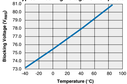
LAA710 Typical Blocking Voltage vs. Temperature
