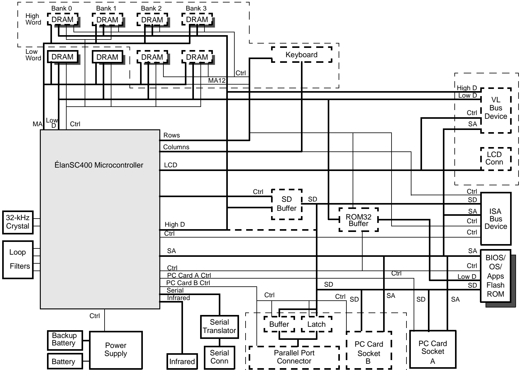
Figure 2. System Diagram with Trade-offs—ÉlanSC400 Microcontroller
