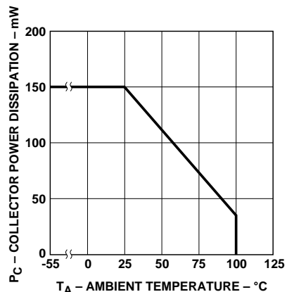
Figure 2. Collector power dissipation vs. temperature.
