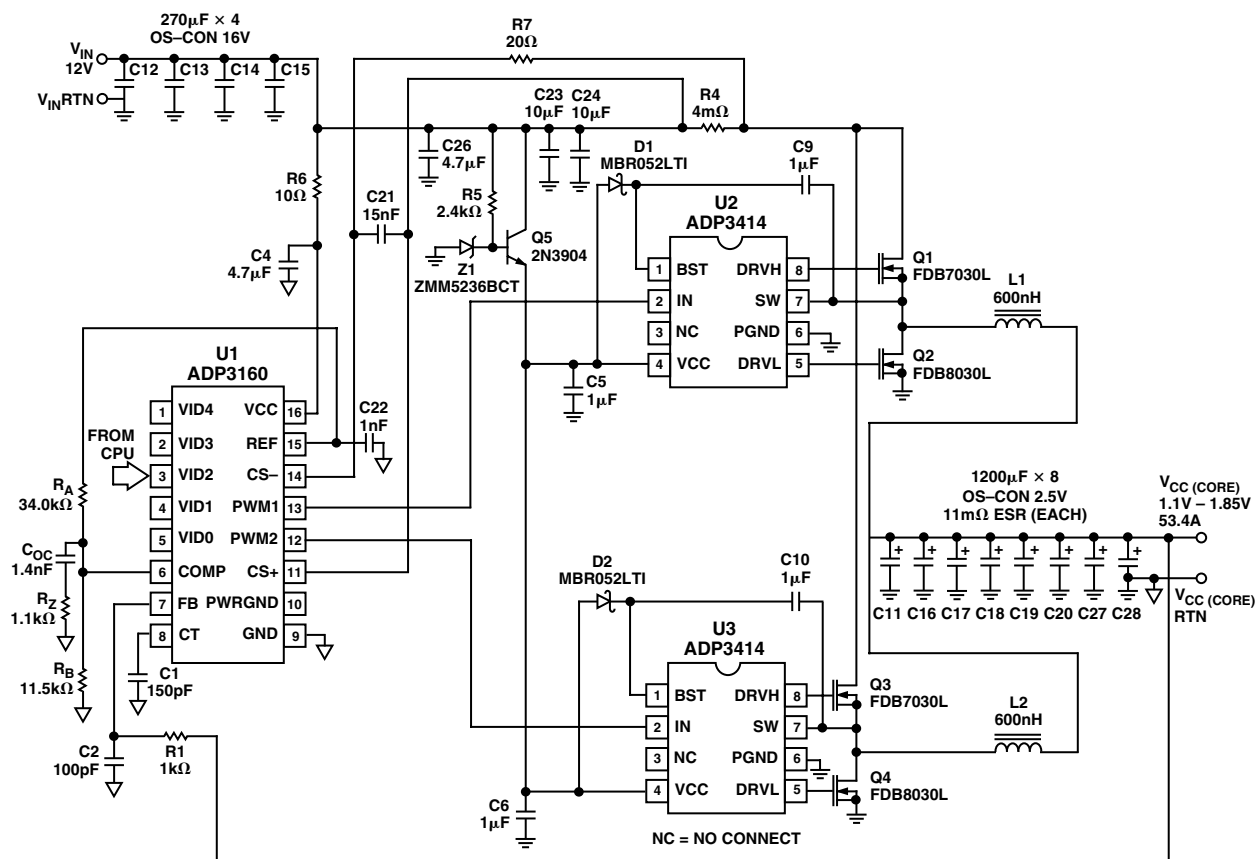
Figure 3. 53.4 A Intel CPU Supply Circuit
