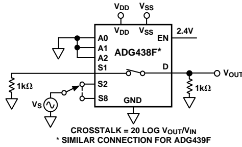
Test Circuit 12. Channel-to-Channel Crosstalk
