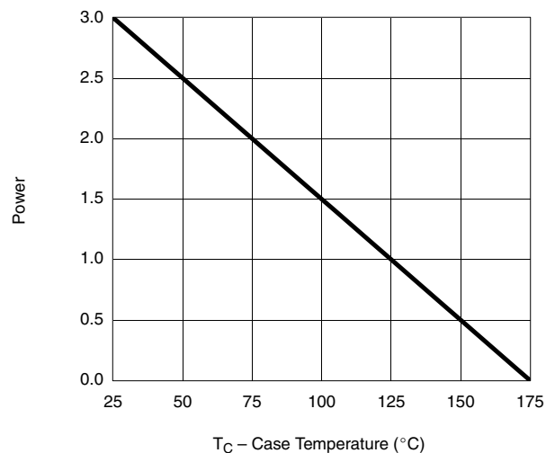
Power De-Rating
