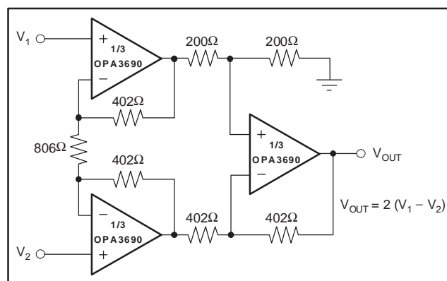
Figure 6. Instrumentation Amplifier
