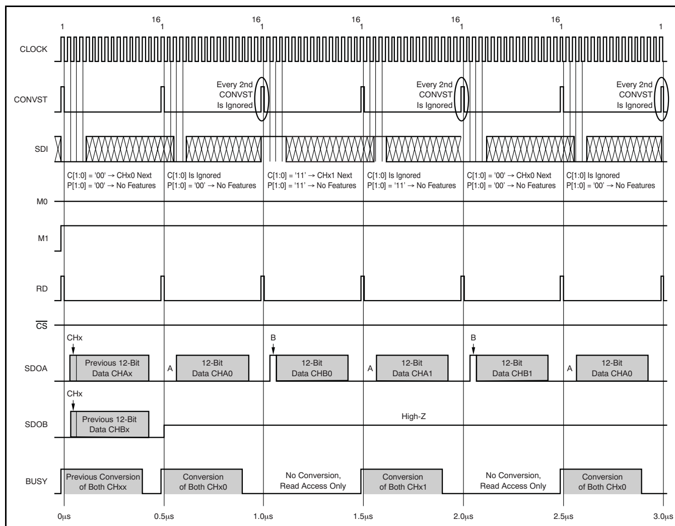
Figure 34. Mode II Timing Diagram (M0 = 0; M1 = 1)
