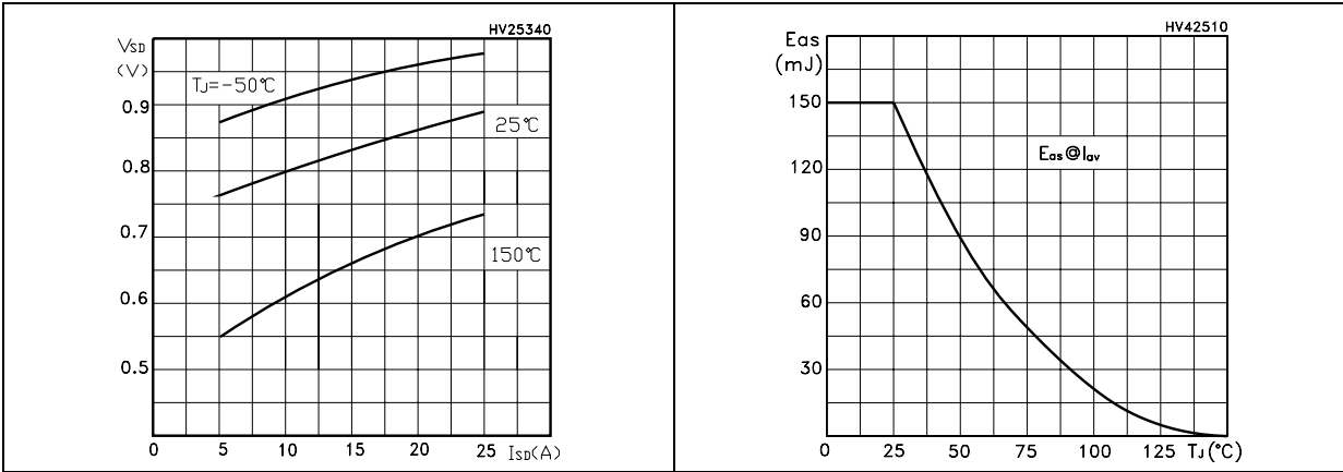
Figure 12. Source-drain diode forward characteristics Figure 13. Avalanche energy vs starting t_i
