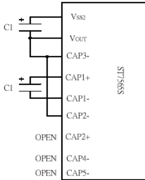
2x step-up voltage circuit
