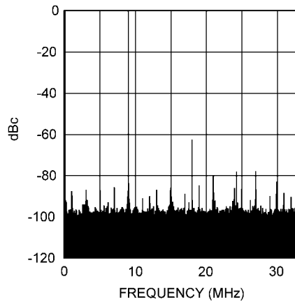
Spectral Response @ 75 MHz Input, -0.5 dBFS
