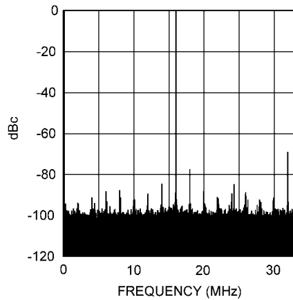
Spectral Response @ 50 MHz Input, -0.5 dBFS
