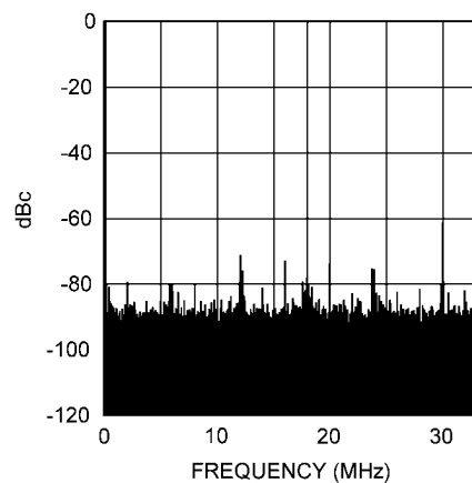
Spectral Response @ 150 MHz Input, -6 dBFS
