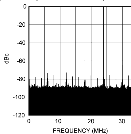
Spectral Response @ 240 MHz Input, -6 dBFS
