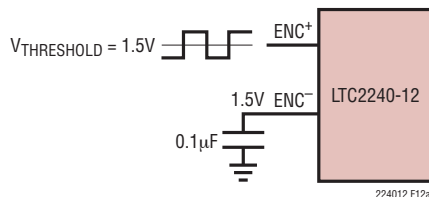
Figure 12a. Single-Ended ENC Drive, Not Recommended for Low Jitter
