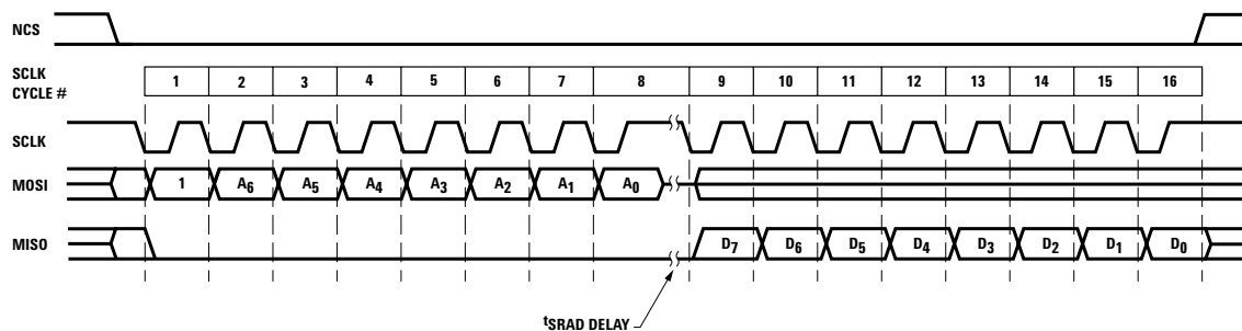
Figure 13. Read operation
