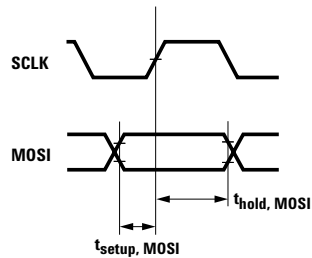
Figure 12. MOSI setup and hold time
