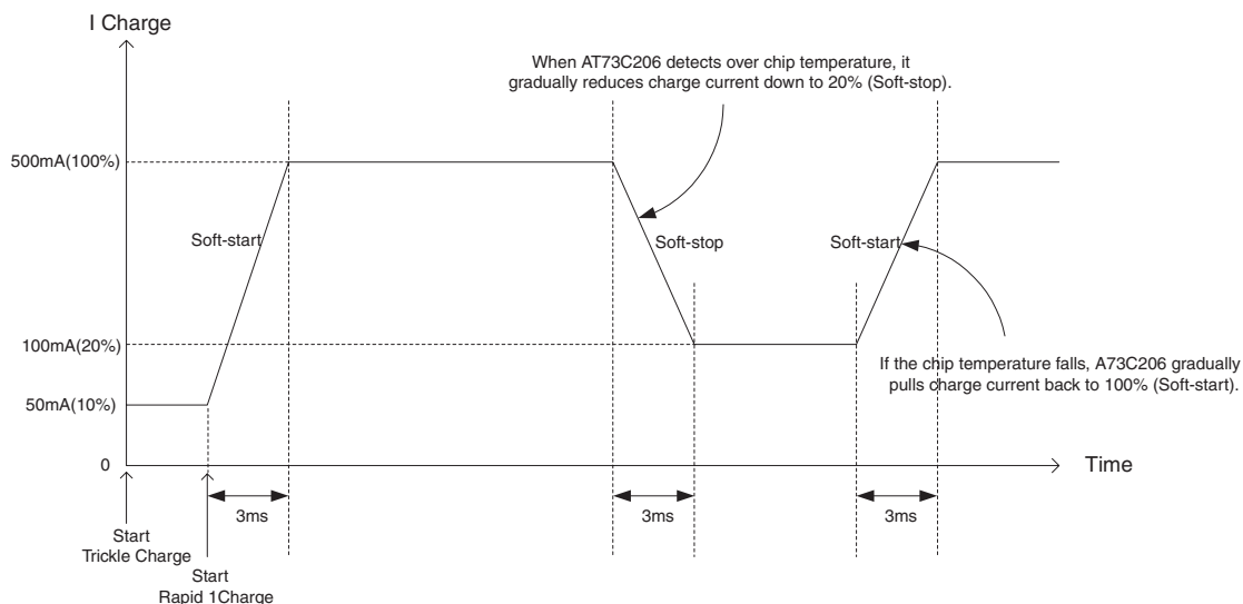
Figure 5-16. Chip Temperature Detection and Soft-start/stop
