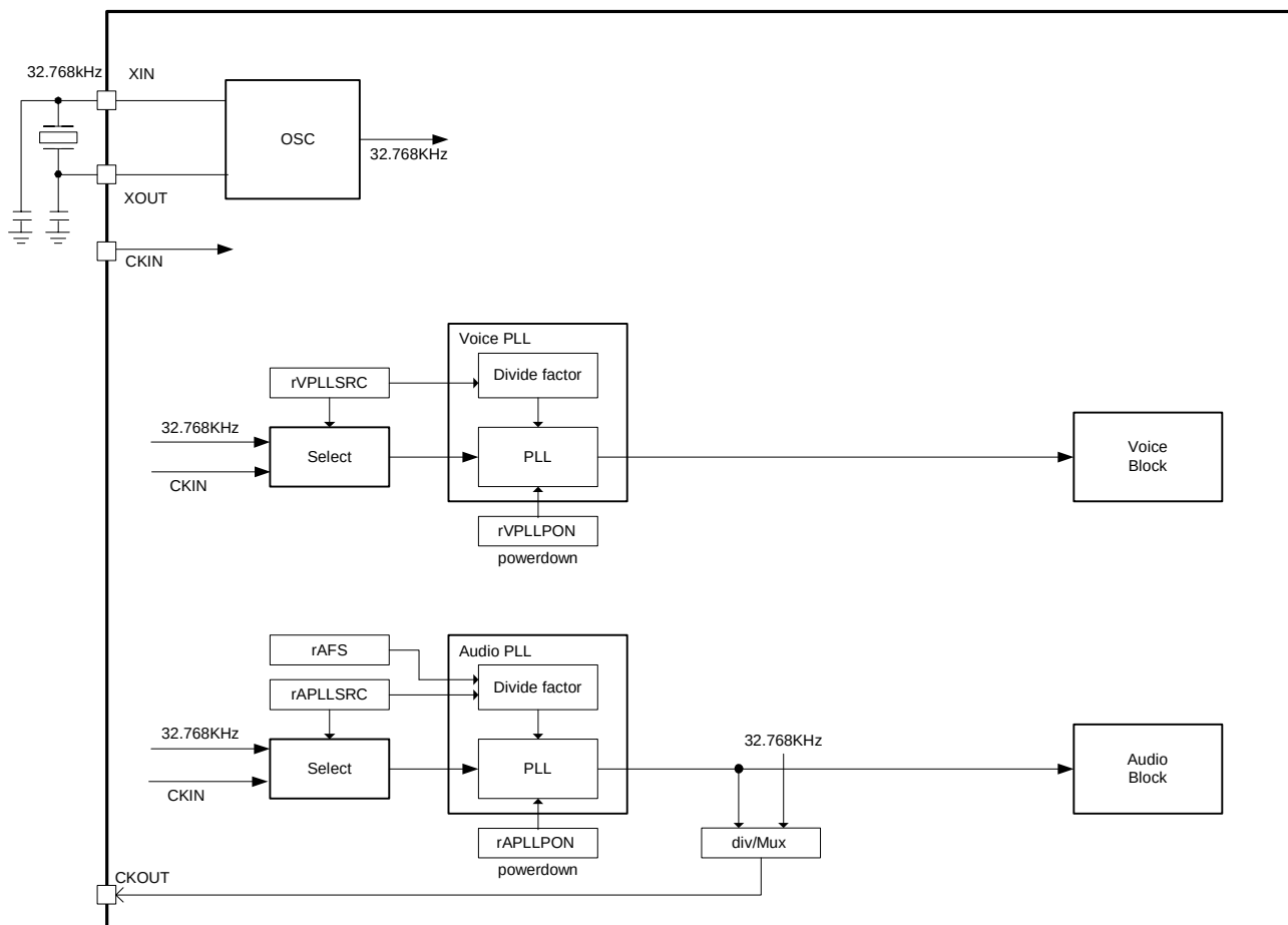
Figure 5-32. Clock Block Diagram
