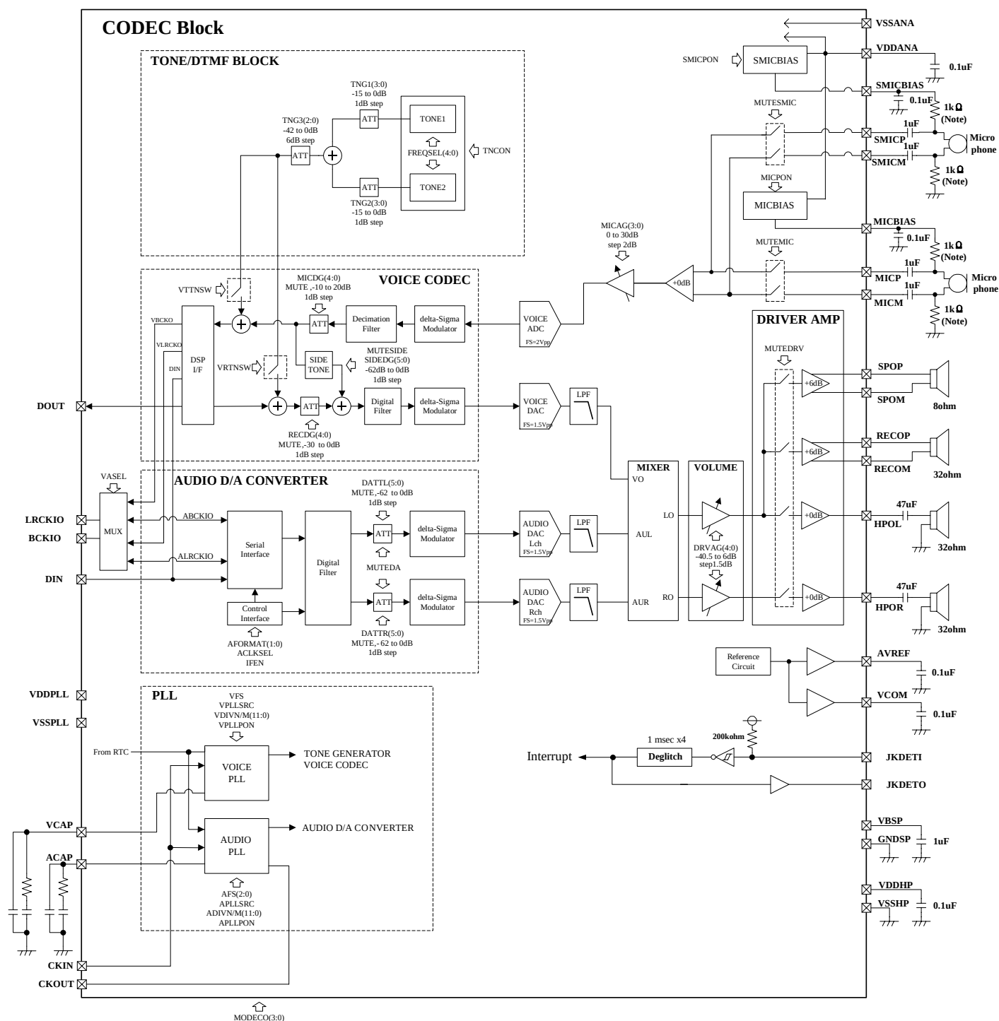
Figure 5-22. CODEC Block Diagram
