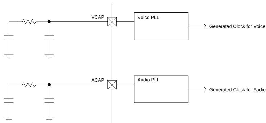
Figure 5-33. PLL Block Diagram
