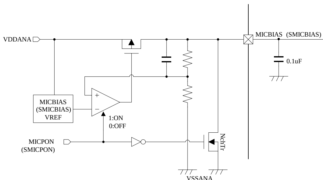
Figure 5-23. MICBIAS, SMICBIAS
