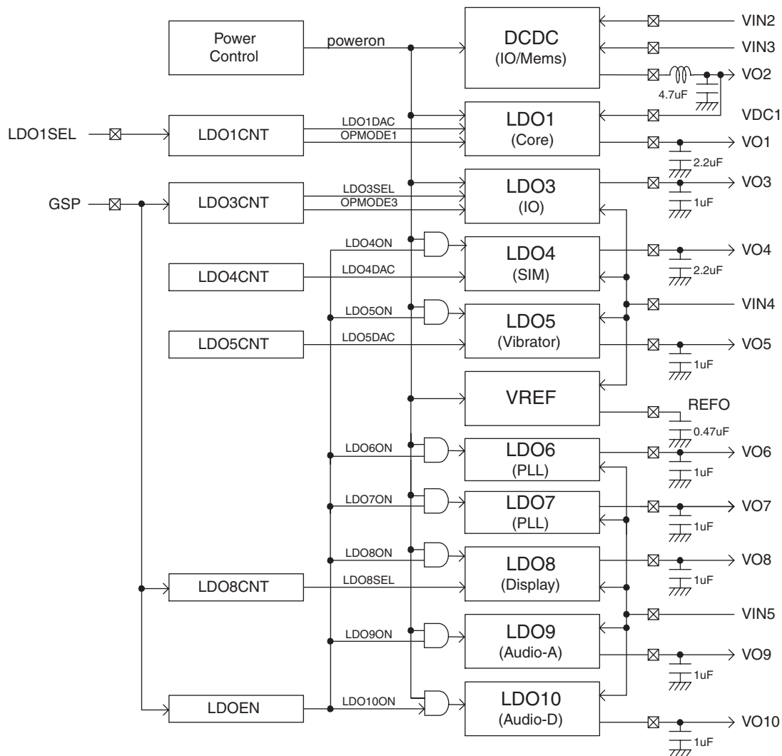
Figure 5-9. LDO Regulator Block Diagram
