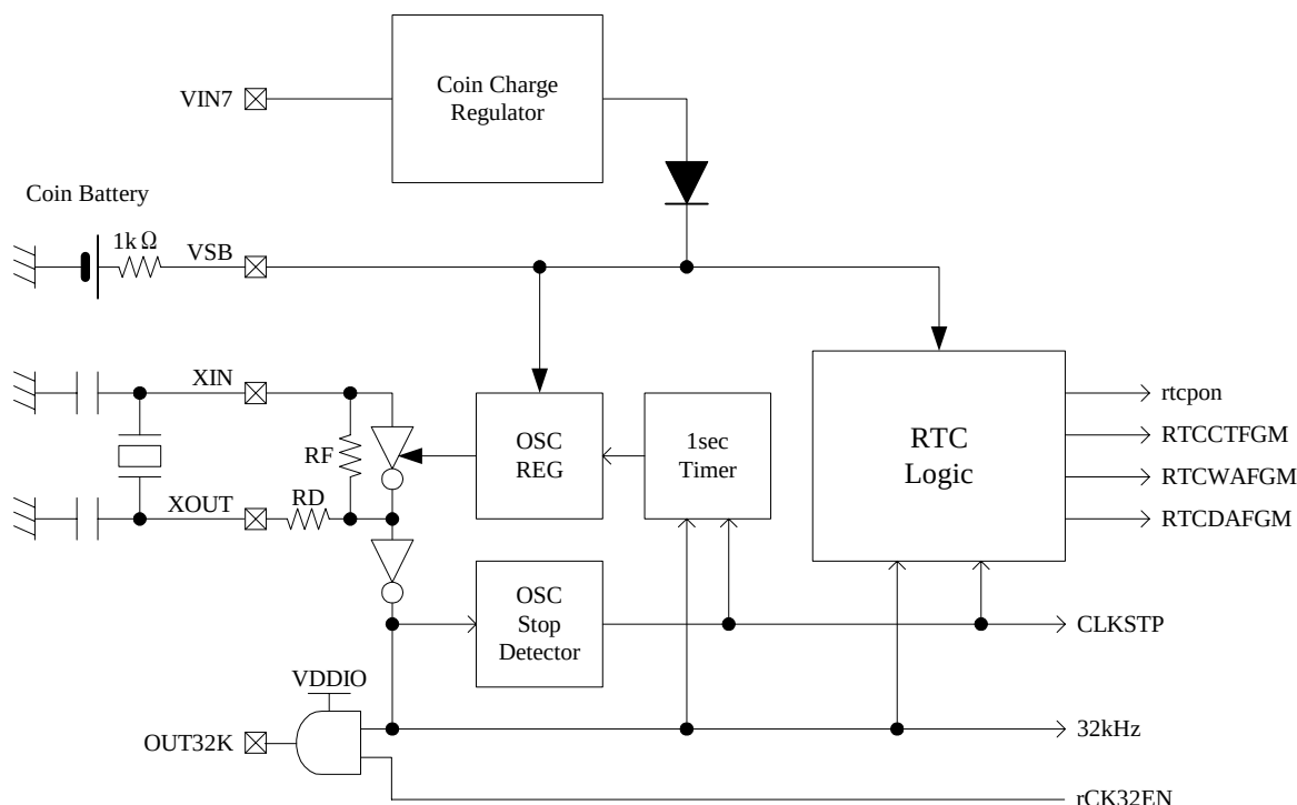
Figure 5-20. RTC Block Diagram
