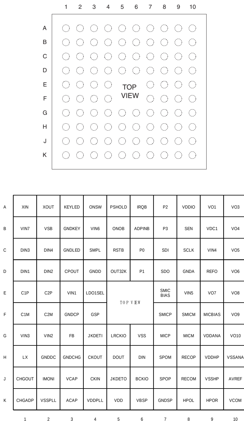
Figure 2-1. Pin Configuration
