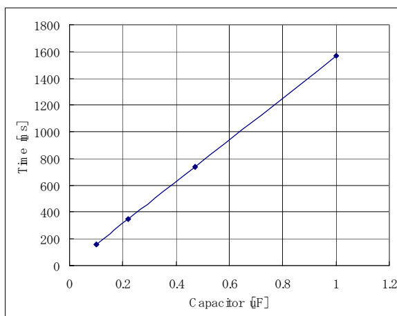
Figure 5-5. SMPL-high-maintain-time when momentary power loss (VIN6 = 3.6V)
