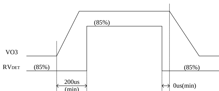
Figure 5-6. VO3 and RESDET Control Timing
