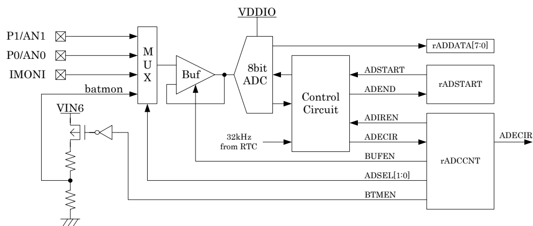
Figure 5-17. ADC Block Diagram
