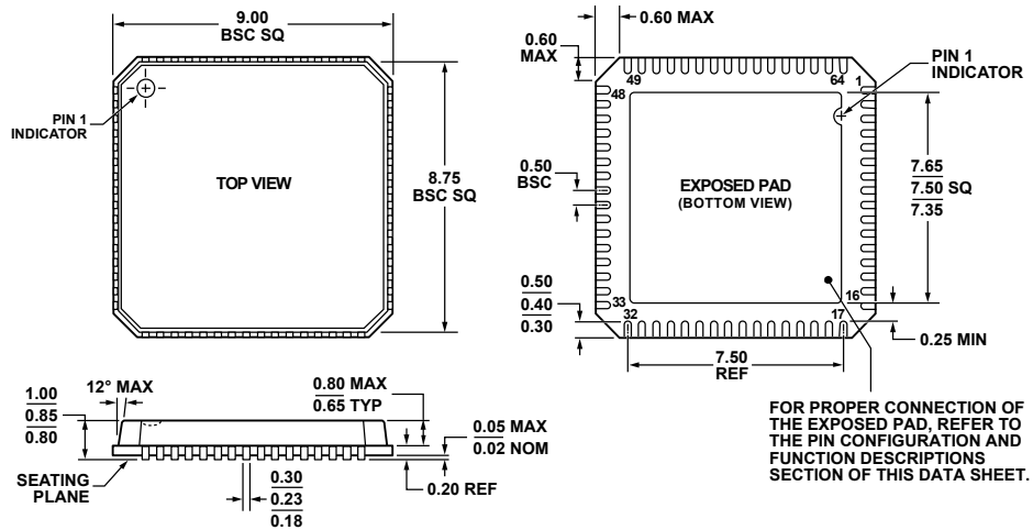
COMPLIANT TO JEDEC STANDARDS MO-220-VMM4 Figure 74. 64-Lead Lead Frame Chip Scale Package [LFCSP_VQ] 9 mm × 9 mm Body, Very Thin Quad (CP-64-6) Dimensions shown in millimeters
