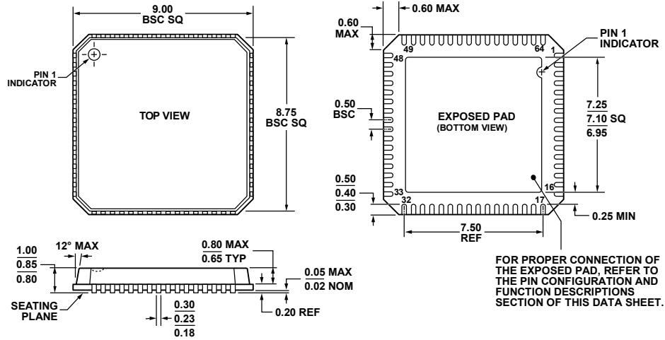
COMPLIANT TO JEDEC STANDARDS MO-220-VMM4 Figure 73. 64-Lead Lead Frame Chip Scale Package [LFCSP_VQ] 9 mm × 9 mm Body, Very Thin Quad (CP-64-3) Dimensions shown in millimeters
