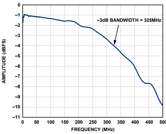
Figure 32. Full-Power Bandwidth vs. Frequency, f_{SAMPLE} = 50 \text{ MSPS}
