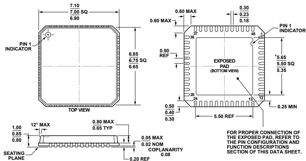
Figure 83. 48 Lead Lead Frame Chip Scale Package [LFCSP_VQ] 7 mm × 7 mm Body, Very Thin Quad (CP-48-8)
