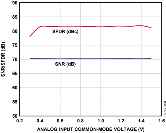
Figure 46. SNR/SFDR vs. Common-Mode Voltage, f_{IN} = 2.4 \text{ MHz} , f_{SAMPLE} = 40 \text{ MSPS}
