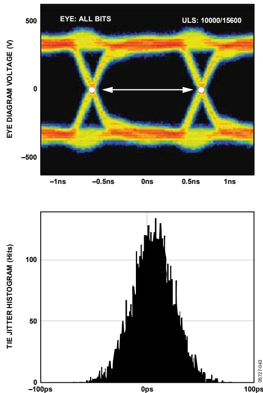
Figure 61. Data Eye for LVDS Outputs in ANSI-644 Mode with Trace Lengths Less than 24 Inches on Standard FR-4, External 100 \Omega Far Termination Only
