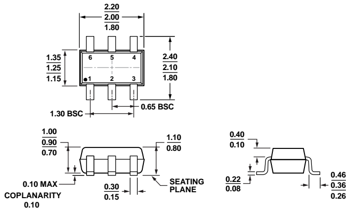
Figure 37. 6-Lead Thin Shrink Small Outline Transistor Package [SC70] (KS-6) Dimensions shown in millimeters
