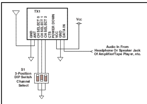
Figure 20: Typical Application: Voice Transmitter
