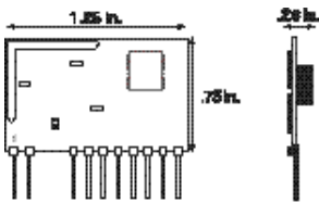
Figure 10: Physical package
