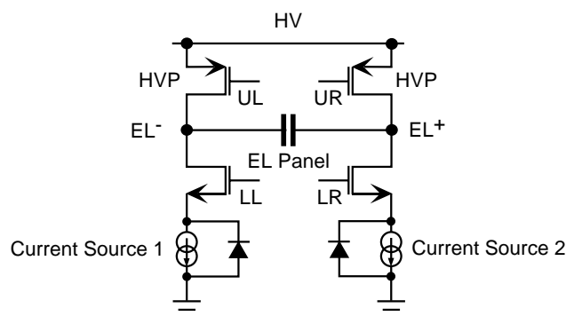
FIGURE 2: H-BRIDGE SCHEMATIC
