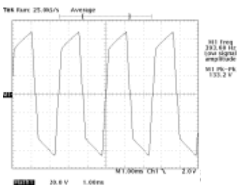
TK65929 Voltage Waveform Across 12 nF Lamp
