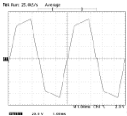
TK65921 Voltage Waveform Across 12 nF Lamp
