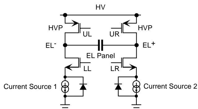
FIGURE 2: H-BRIDGE SCHEMATIC
