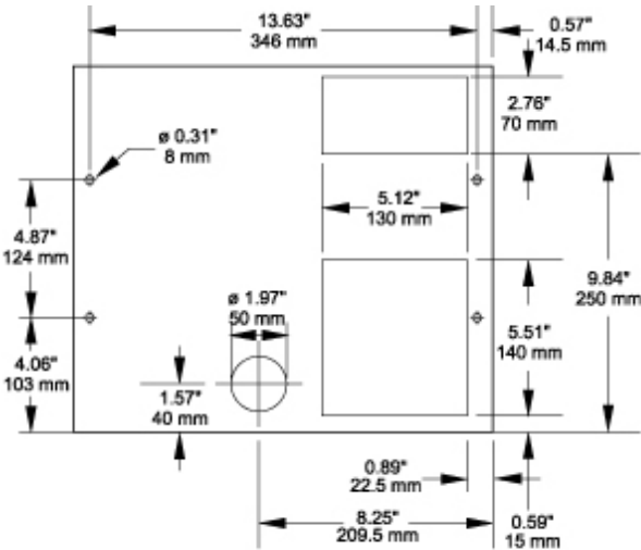
Drilling Template
